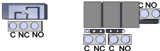
Schema 6: EXP Relay ed EXP Relay3
